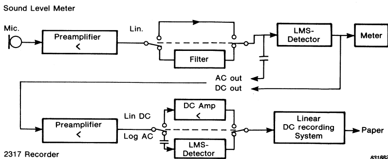
Fig. 1. General description of Measuring System
