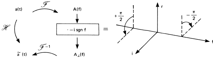
Fig. 3. The effect of the Hilbert Transform of a time signal as seen in the frequency domain
