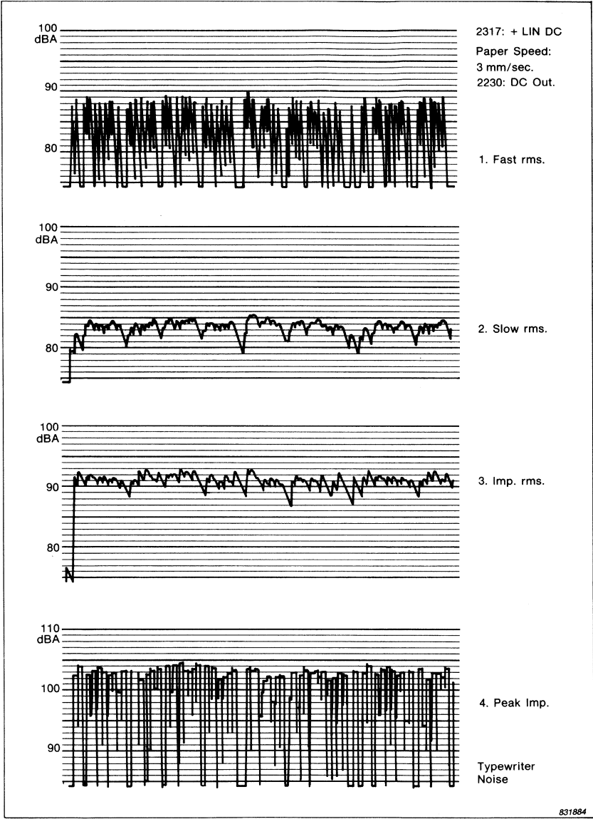
Fig. 3. Typewriter Noise recorded in different modes
