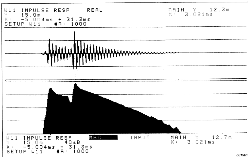
Fig. 8. Two presentations of the Impulse Response of a physical system. Upper part: Traditional method. Lower part: Envelope calculated using the Hilbert Transform
