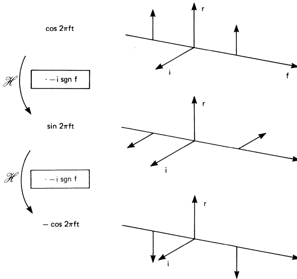
Fig. 4. Hilbert Transforms of a sinusoid as seen in the frequency domain
