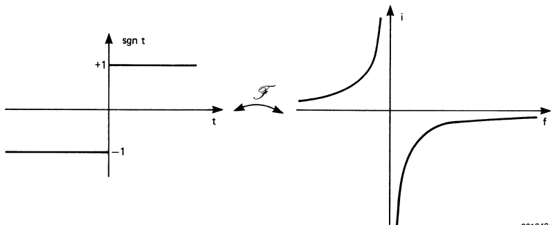
Fig. 2. Fourier Transform of \text{sgn } t
