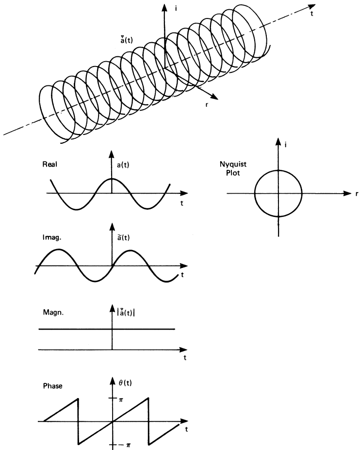
Fig. 6. The analytic signal of a cosine
