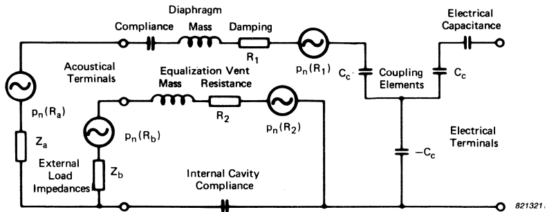
Fig. 2. Model of Condenser Microphone Cartridge
