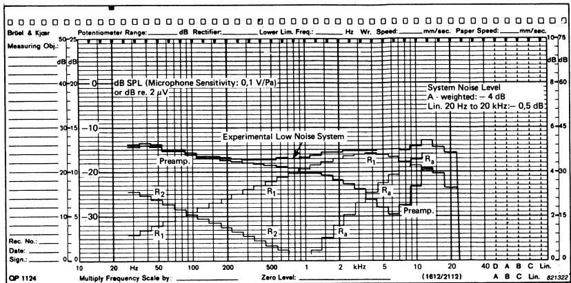
Fig. 4. Third octave analyses of the noise produced by the Experimental Low Noise Microphone System and of the individual elements
