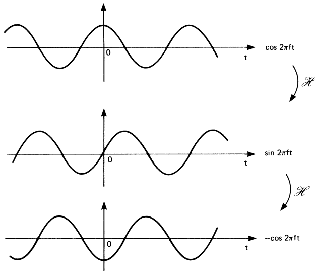
Fig. 1. Hilbert Transforms of a sinusoid
