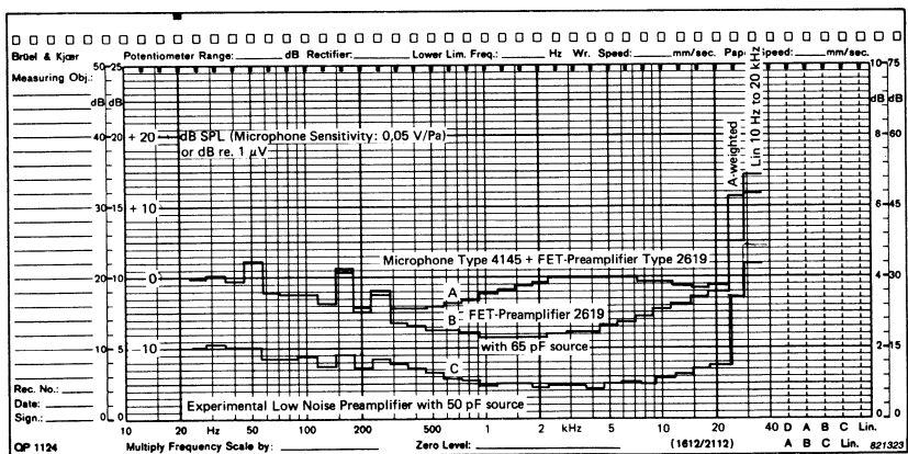
Fig. 1. Third octave analysis of Preamplifier output Noise Voltages
