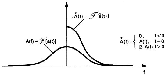
Fig. 7. The spectrum, A(f) , of a real time signal, a(t) , compared to the spectrum, \tilde{A}(f) , of the corresponding analytic signal, \tilde{a}(t)
