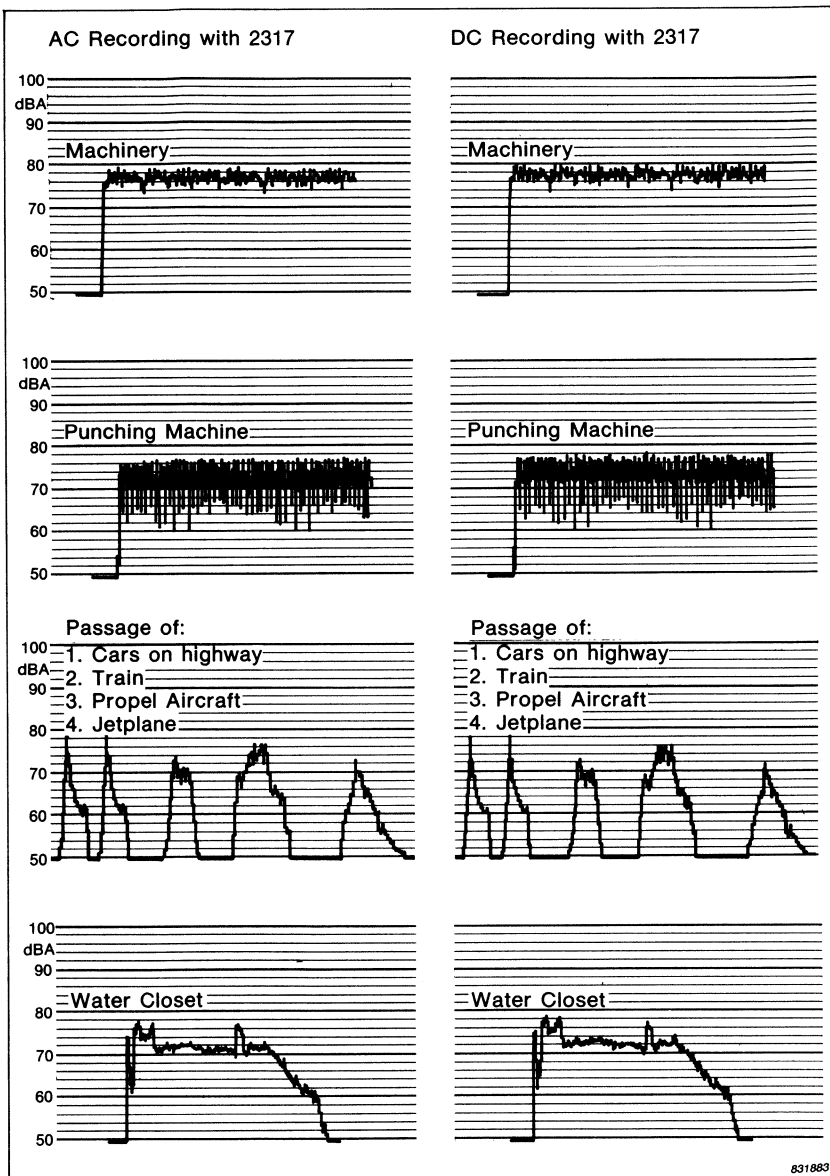
Fig. 2. Examples of Noise Recordings
